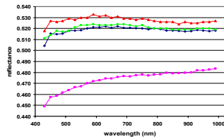
Reflectance of 52% Tarp
