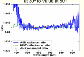
Ratio of Radiance (or Reflectance) at 30° to Value at 50°
