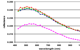
Reflectance of 22% Tarp
