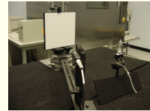
Radiance Values Measured with ASD FieldSpec Pro
