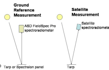
Measuring tarp signal with ASD FieldSpec Pro during overpass
