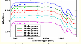
NIST Reflectance Values for Varying Angles of Incidence
